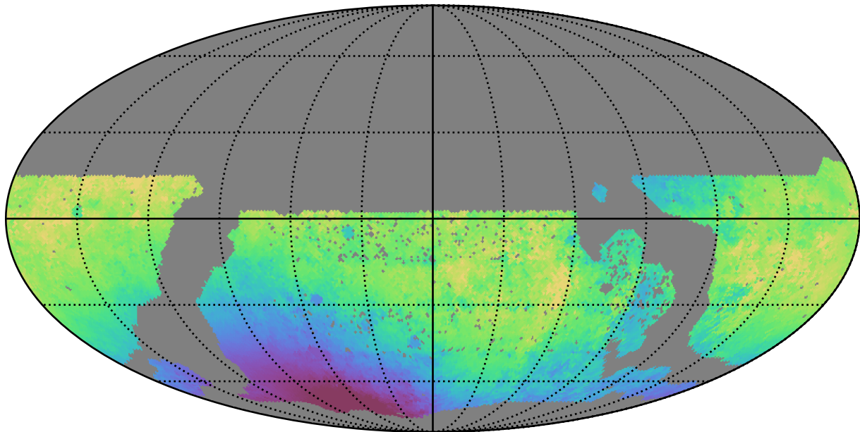
too_combined_s0.0_v3.4_10yrs WFD g band: Median solarElong
