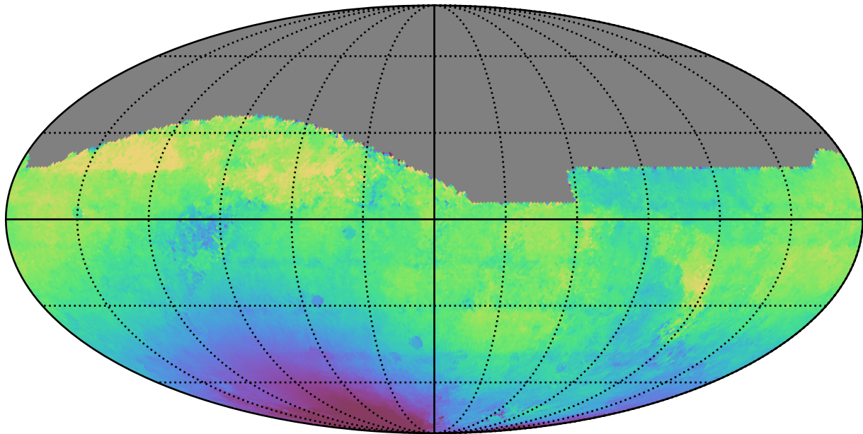
too_combined_s0.0_v3.4_10yrs All sky r band: Median solarElong
