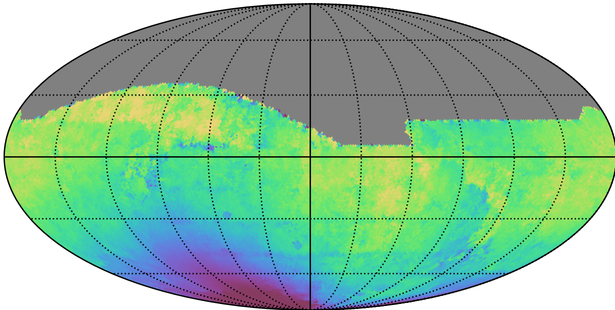
too_combined_s0.0_v3.4_10yrs All sky i band: Median solarElong
