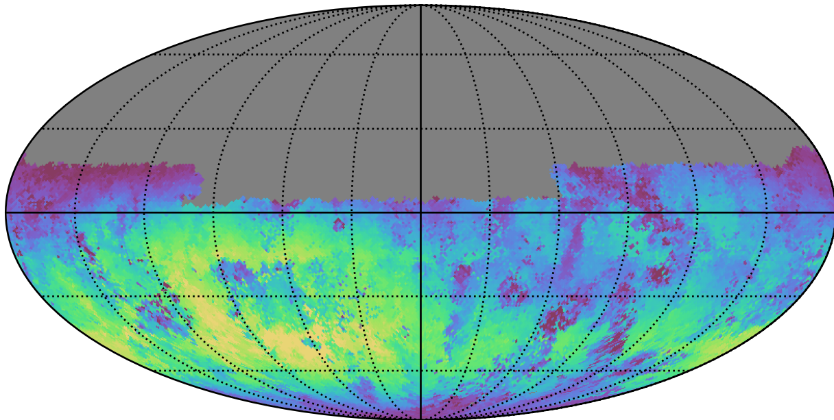
too_combined_s0.0_v3.4_10yrs Yr 1 u band: Median skyBrightness
