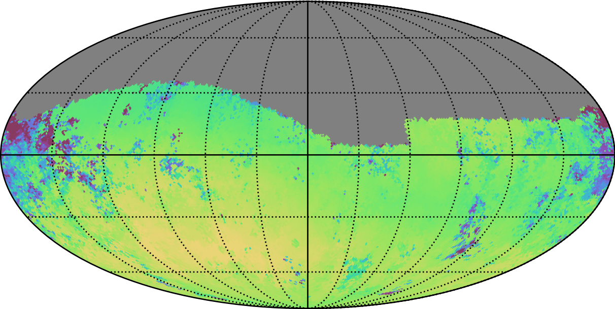
too_combined_s0.0_v3.4_10yrs Yr 1 g band: Median skyBrightness
