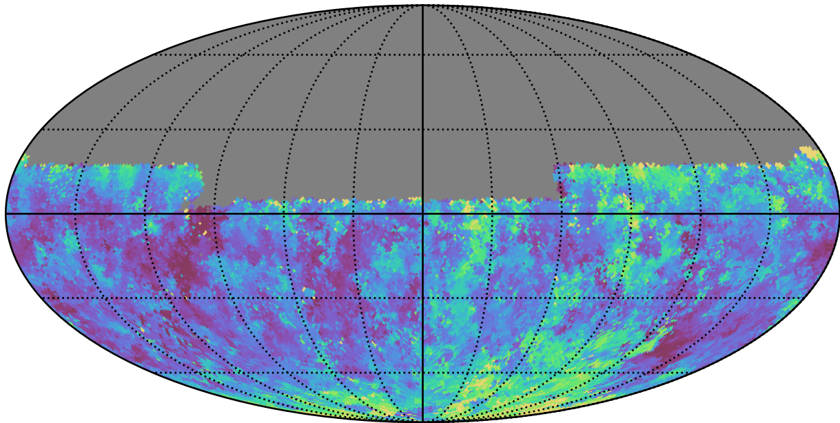
too_combined_s0.0_v3.4_10yrs Yr 1 y band: Median seeingEff
