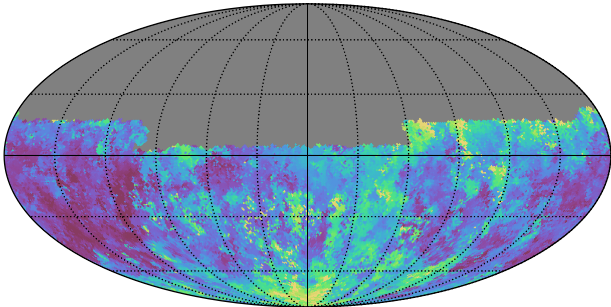
too_combined_s0.0_v3.4_10yrs Yr 1 u band: Median seeingEff
