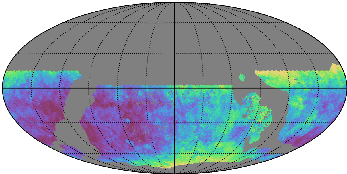
too_combined_s0.0_v3.4_10yrs WFD y band: Median seeingEff
