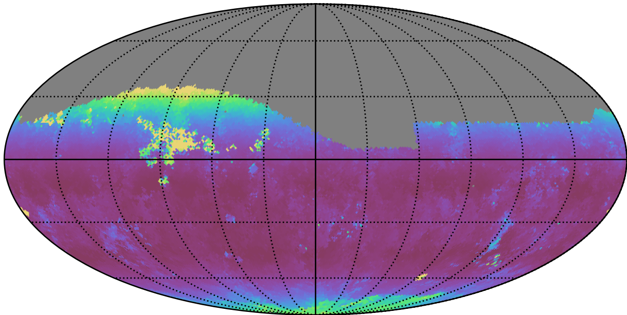
too_combined_s0.0_v3.4_10yrs Yr 1 z band: Median airmass
