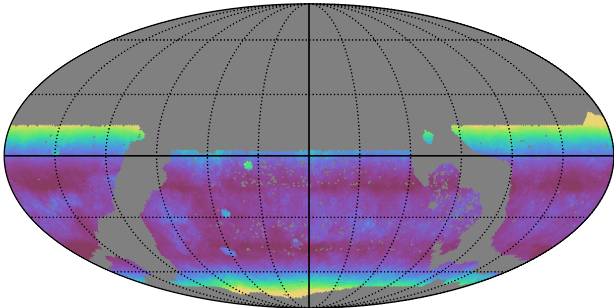
too_combined_s0.0_v3.4_10yrs WFD z band: Median airmass
