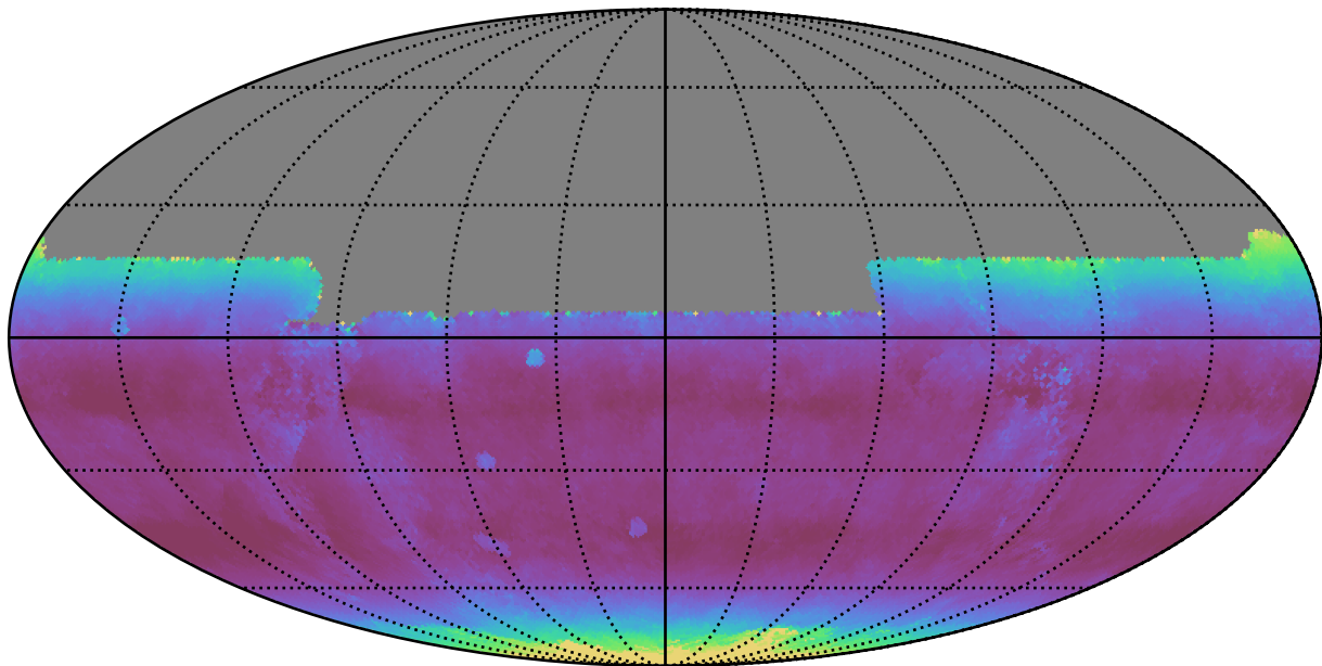
too_combined_s0.0_v3.4_10yrs All sky y band: Median airmass
