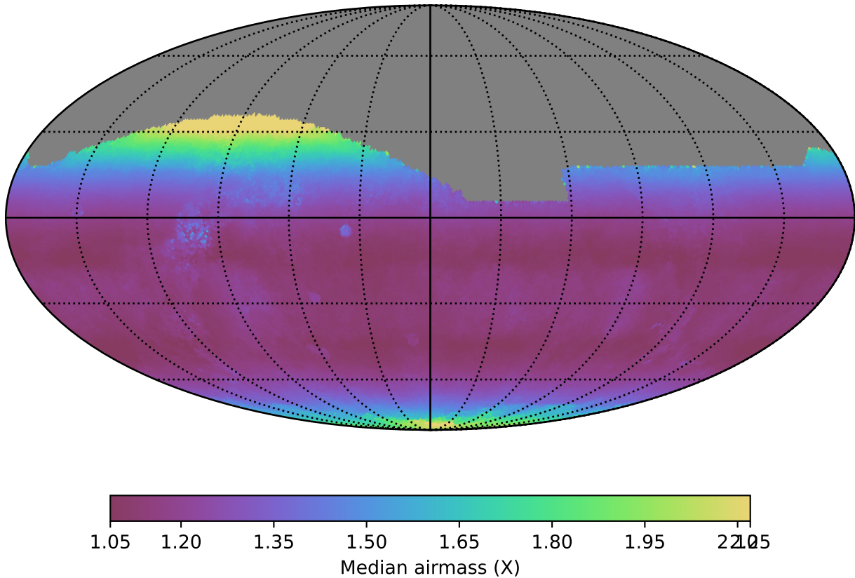
too_combined_s0.0_v3.4_10yrs All sky r band: Median airmass
