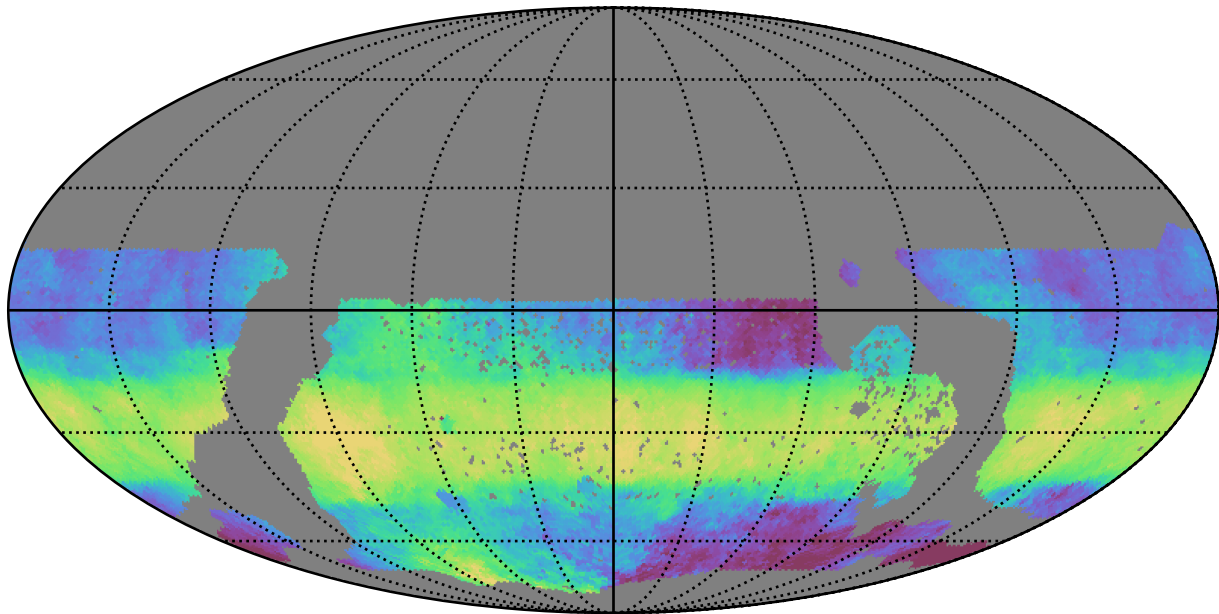
too_combined_s0.0_v3.4_10yrs WFD z band: Median HA
