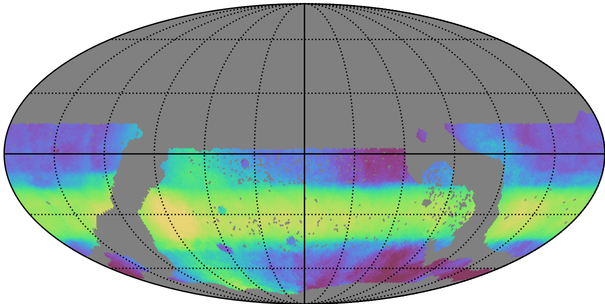
too_combined_s0.0_v3.4_10yrs WFD all bands: Median HA
