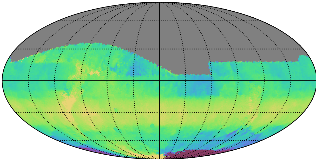
too_combined_s0.0_v3.4_10yrs All sky z band: Median HA
