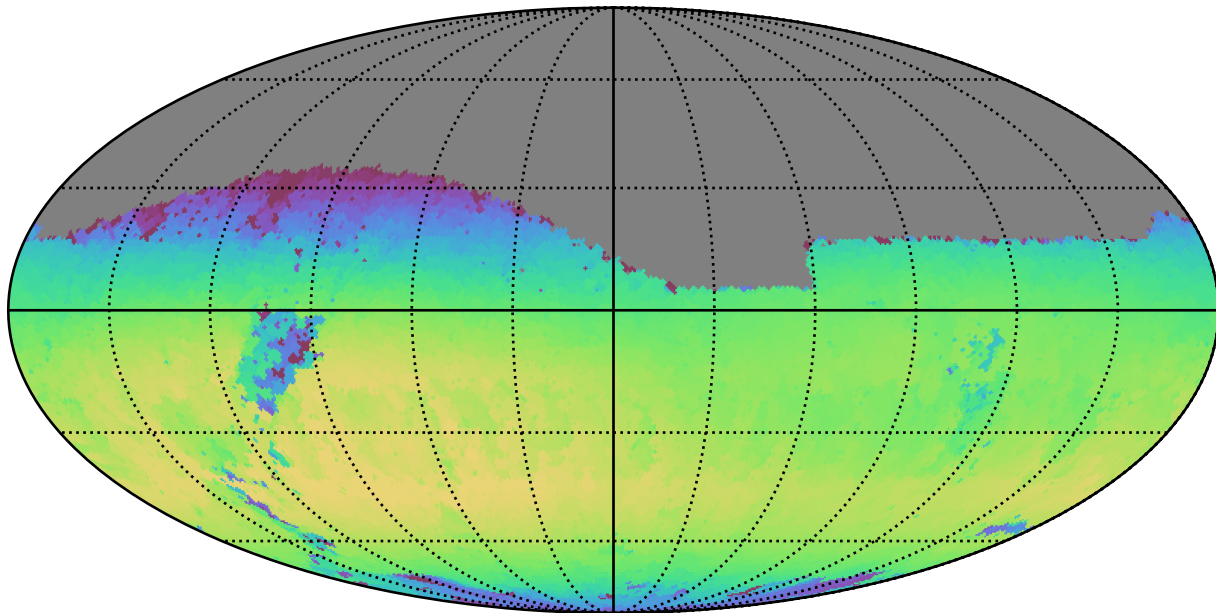
too_combined_s0.0_v3.4_10yrs Yr 1 i band: Max skyBrightness
