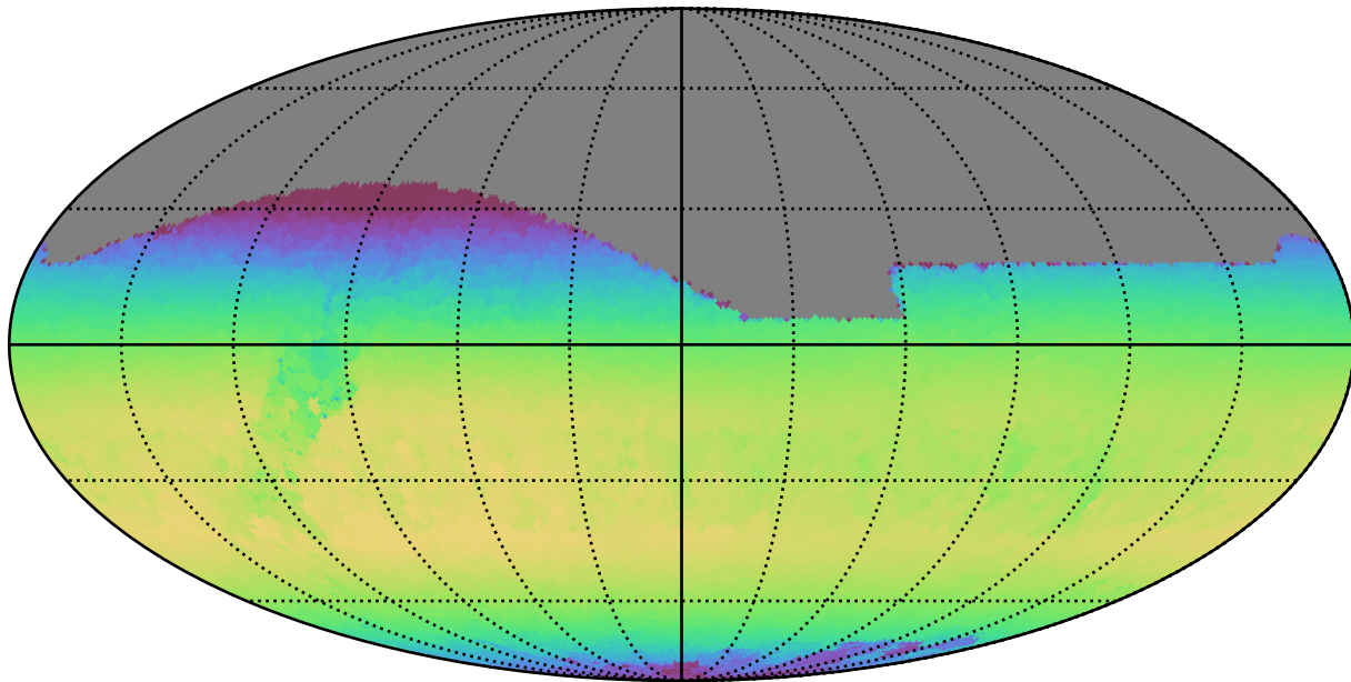
too_combined_s0.0_v3.4_10yrs All sky z band: Max skyBrightness
