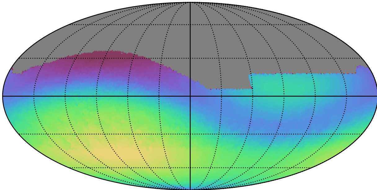
too_combined_s0.0_v3.4_10yrs All sky g band: Max skyBrightness
