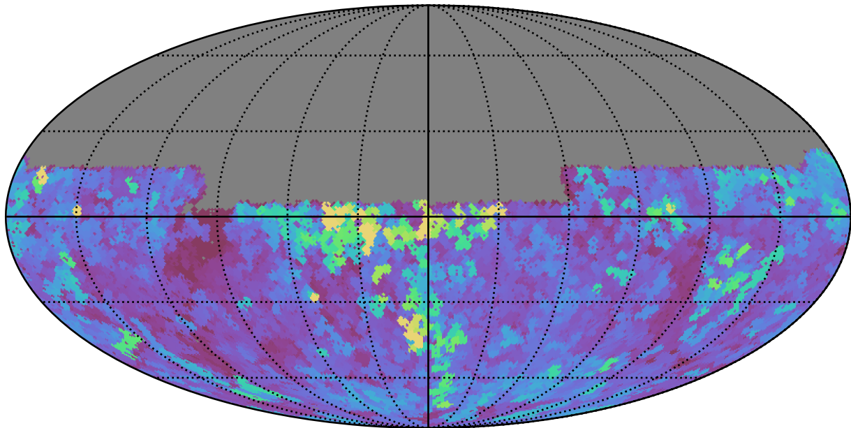
too_combined_s0.0_v3.4_10yrs Yr 1 y band: Max seeingGeom
