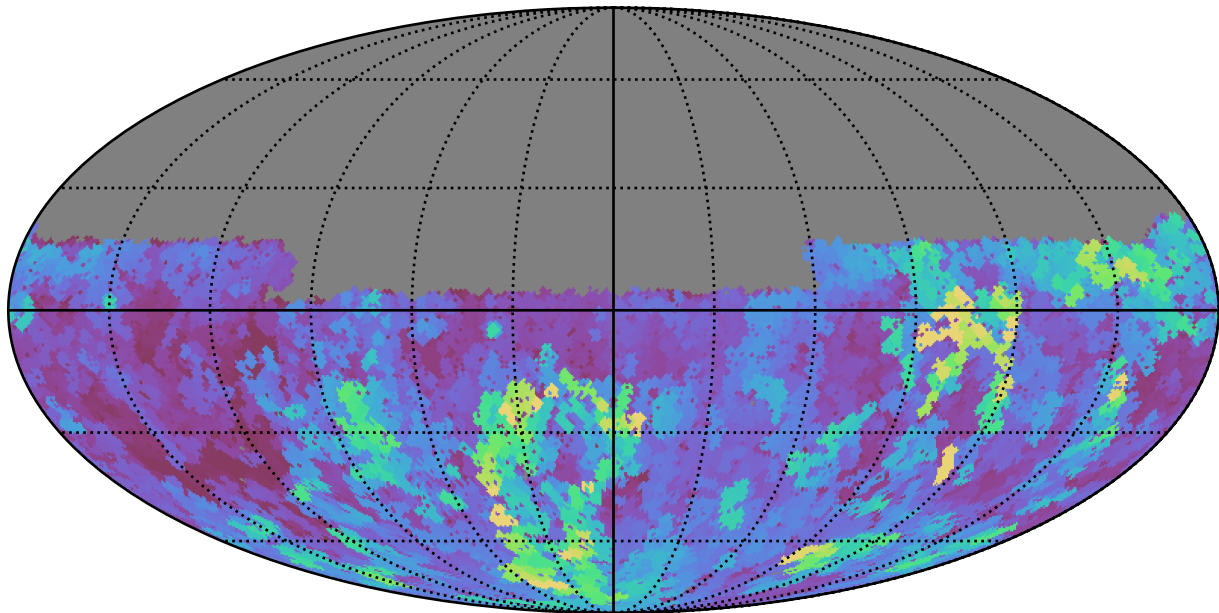
too_combined_s0.0_v3.4_10yrs Yr 1 u band: Max seeingGeom
