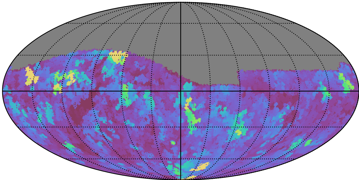
too_combined_s0.0_v3.4_10yrs Yr 1 i band: Max seeingGeom
