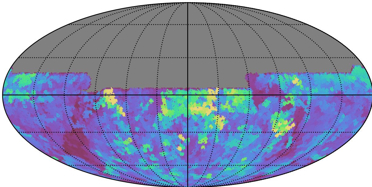
too_combined_s0.0_v3.4_10yrs All sky u band: Max seeingEff
