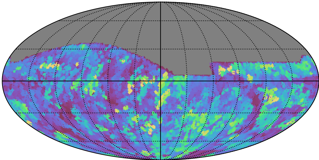
too_combined_s0.0_v3.4_10yrs All sky r band: Max seeingEff
