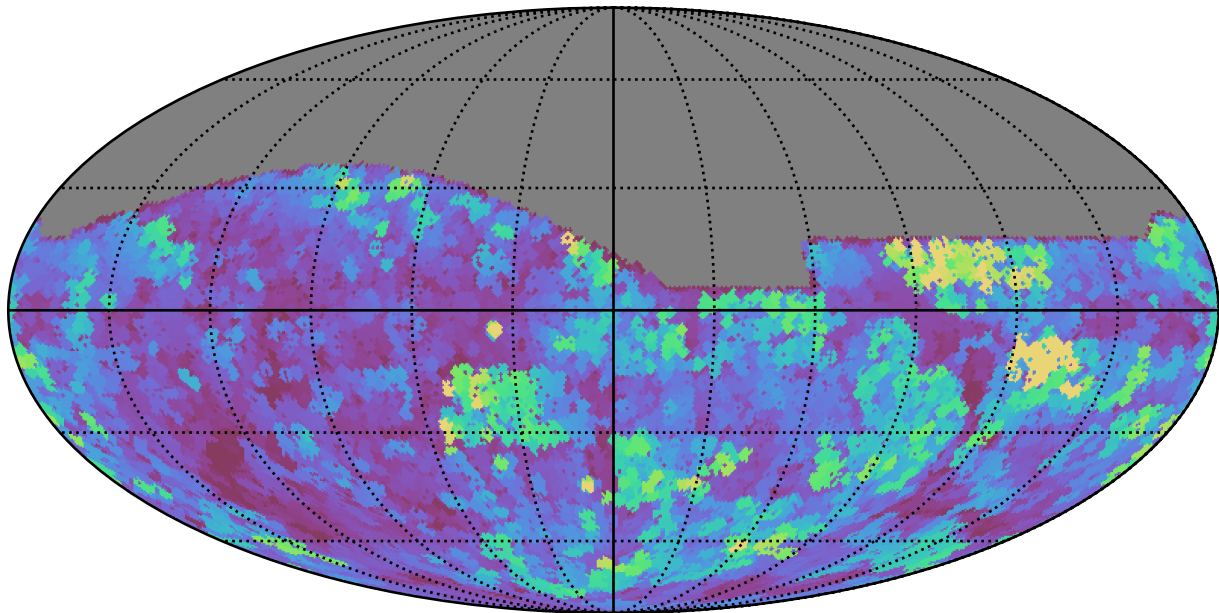
too_combined_s0.0_v3.4_10yrs All sky g band: Max seeingEff
