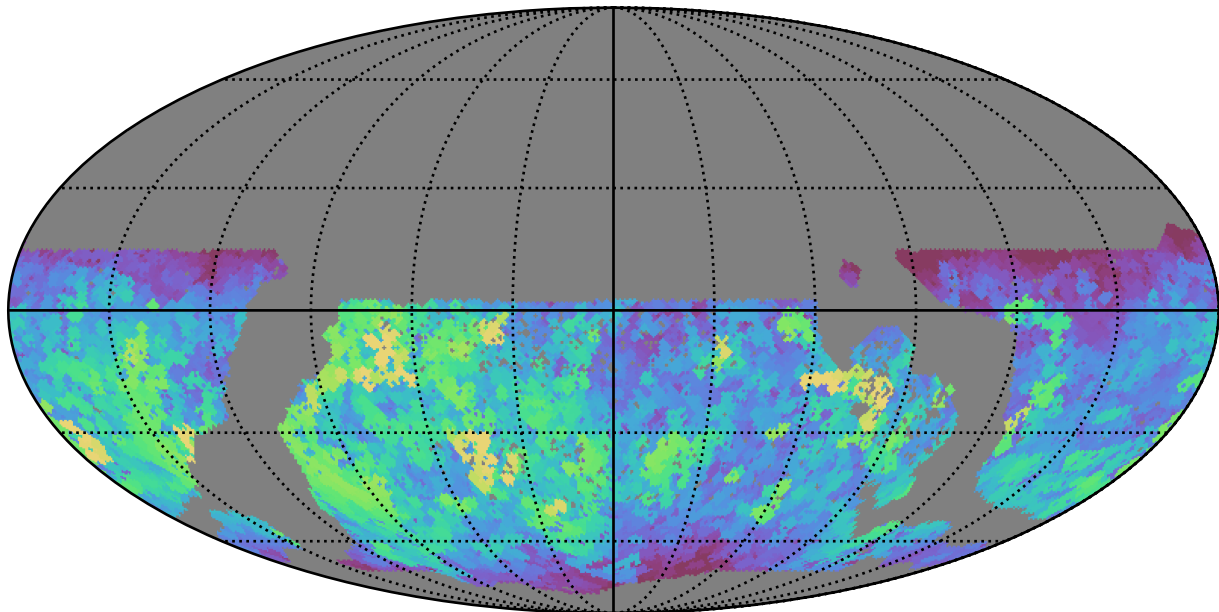
too_combined_s0.0_v3.4_10yrs WFD i band: Max saturation_mag
