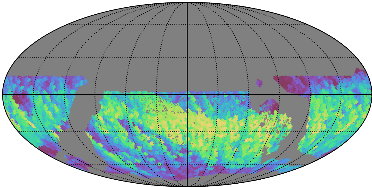
too_combined_s0.0_v3.4_10yrs WFD i band: Max normairmass
