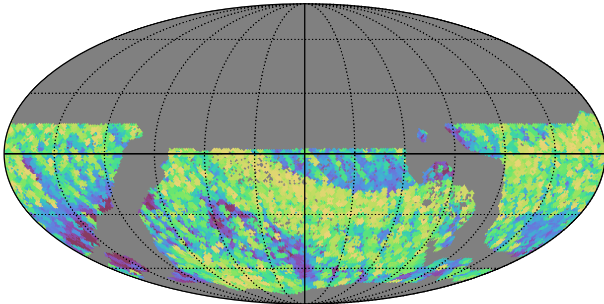
too_combined_s0.0_v3.4_10yrs WFD all bands: Max airmass
