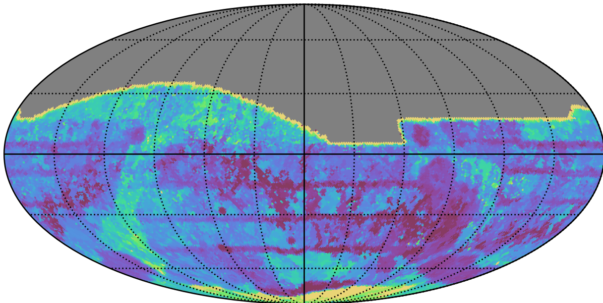
too_combined_s0.0_v3.4_10yrs All sky all bands: Max Inter-Night Gap
