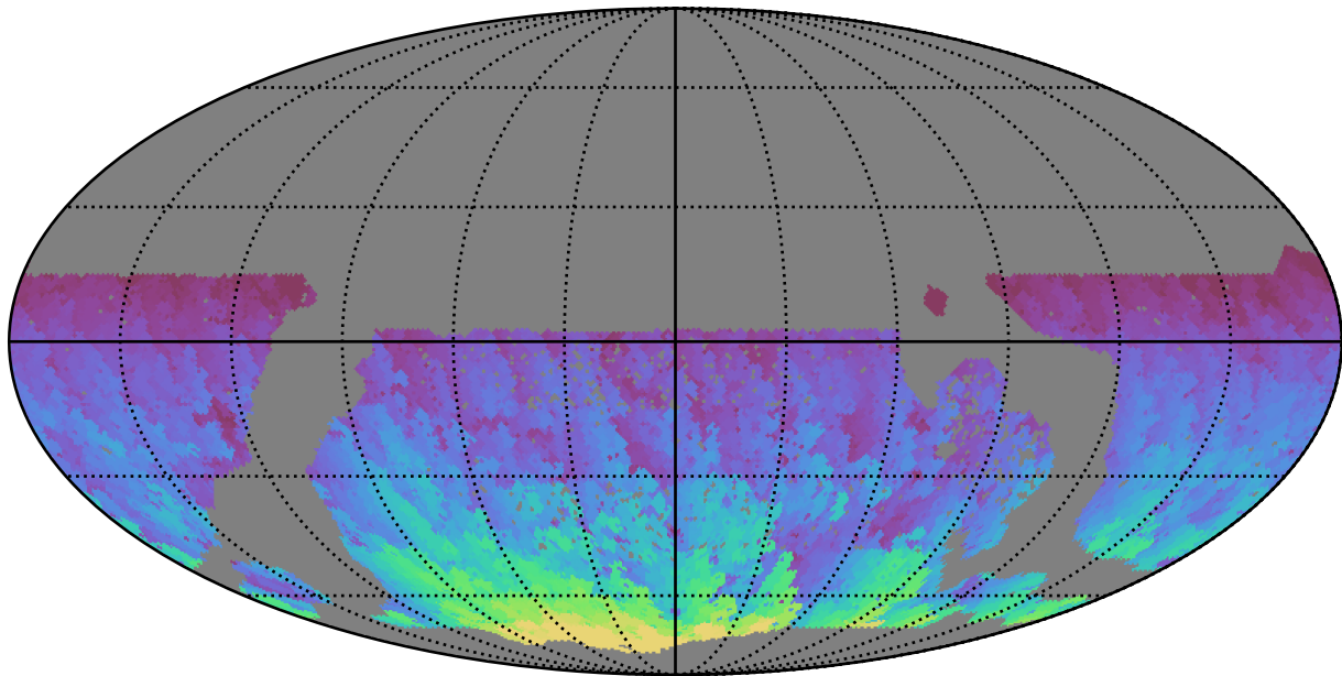
too_combined_s0.0_v3.4_10yrs WFD y band: Max HA
