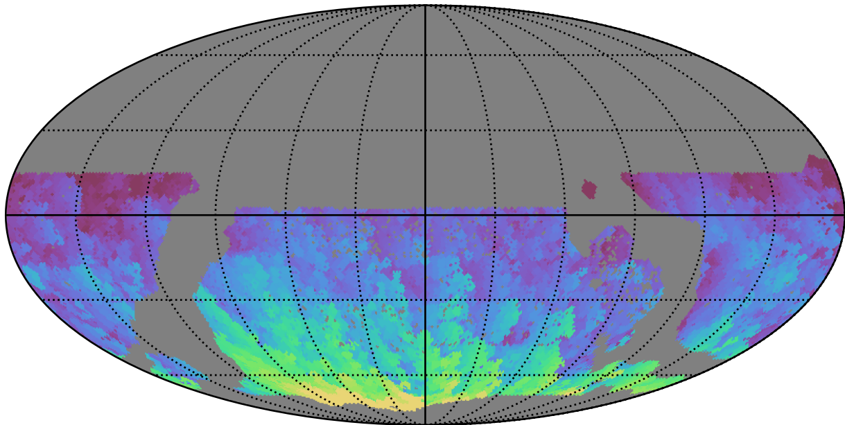
too_combined_s0.0_v3.4_10yrs WFD r band: Max HA
