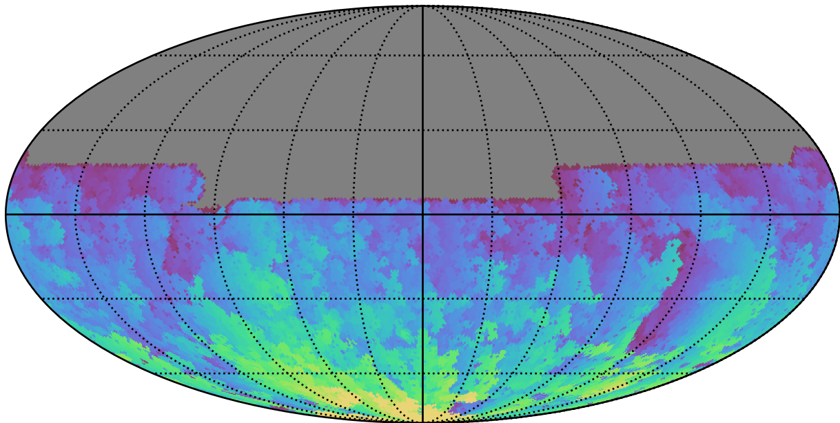
too_combined_s0.0_v3.4_10yrs All sky u band: Max HA
