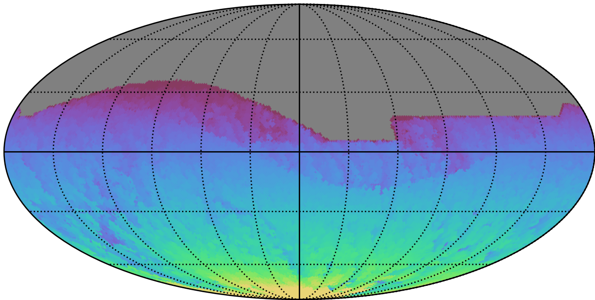
too_combined_s0.0_v3.4_10yrs All sky all bands: Max HA
