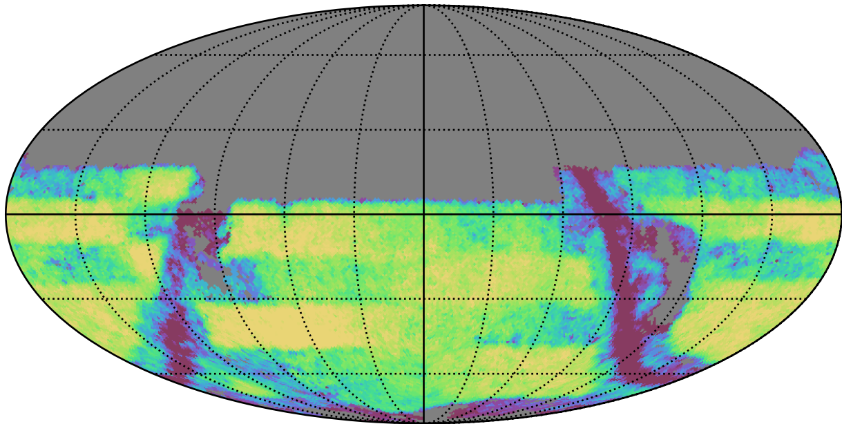
too_combined_s0.0_v3.4_10yrs Yr 3-4 y band: Exgal_CoaddM5
