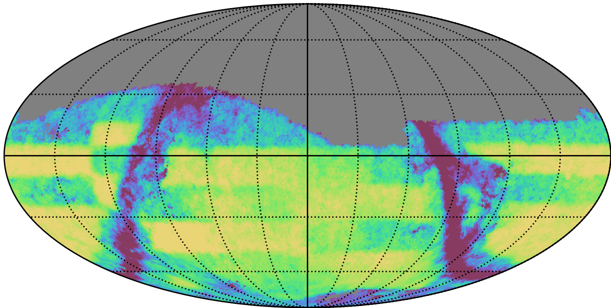
too_combined_s0.0_v3.4_10yrs Yr 3-4 i band: Exgal_CoaddM5
