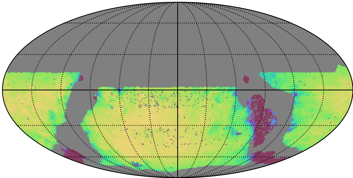
too_combined_s0.0_v3.4_10yrs WFD u band: Exgal_CoaddM5
