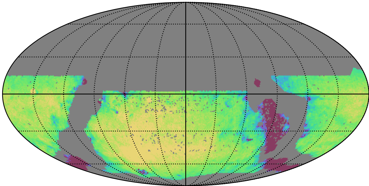
too_combined_s0.0_v3.4_10yrs WFD g band: Exgal_CoaddM5
