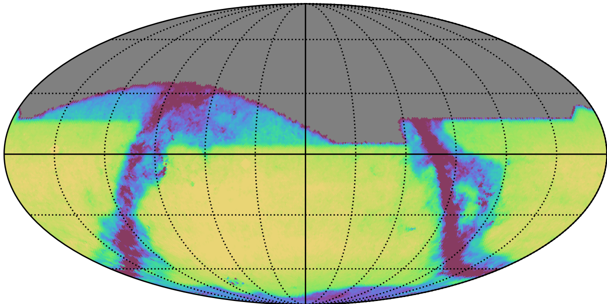
too_combined_s0.0_v3.4_10yrs All sky z band: Exgal_CoaddM5
