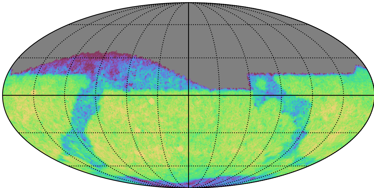
too_combined_s0.0_v3.4_10yrs Yr 1 z band: CoaddM5
