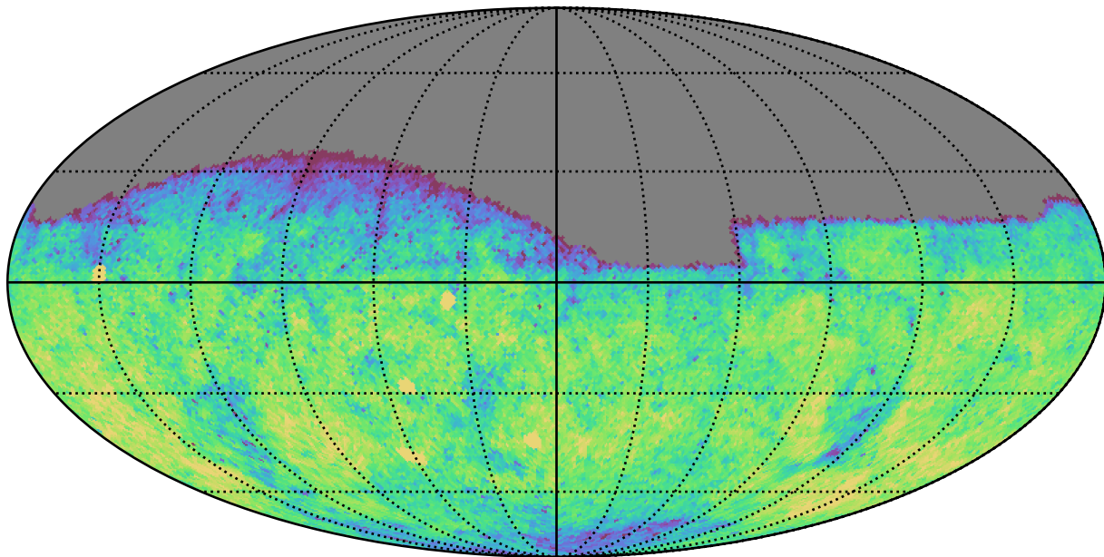
too_combined_s0.0_v3.4_10yrs Yr 1 g band: CoaddM5
