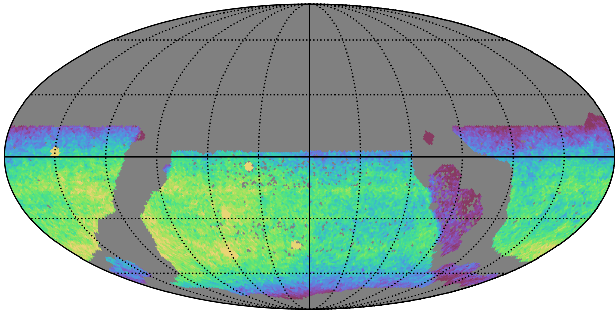
too_combined_s0.0_v3.4_10yrs WFD y band: CoaddM5
