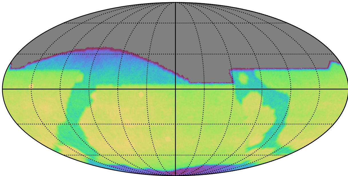
too_combined_s0.0_v3.4_10yrs All sky r band: CoaddM5
