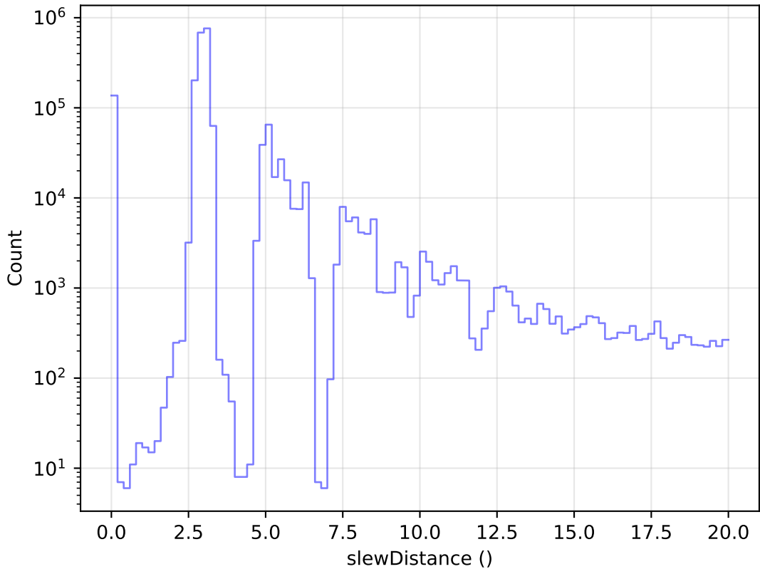
too_combined_s0.0_v3.4_10yrs All visits: Zoom Slew Distance Histogram
