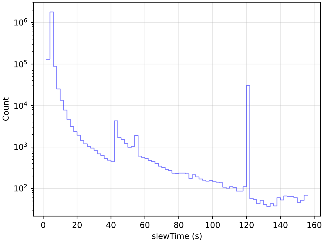
too_combined_s0.0_v3.4_10yrs All visits: Slew Time Histogram
