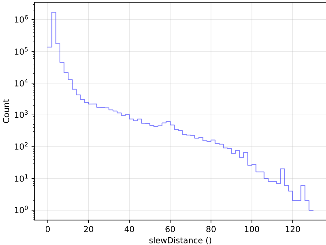
too_combined_s0.0_v3.4_10yrs All visits: Slew Distance Histogram
