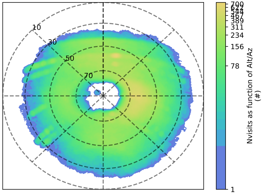
too_combined_s0.0_v3.4_10yrs u: Nvisits as function of Alt/Az
