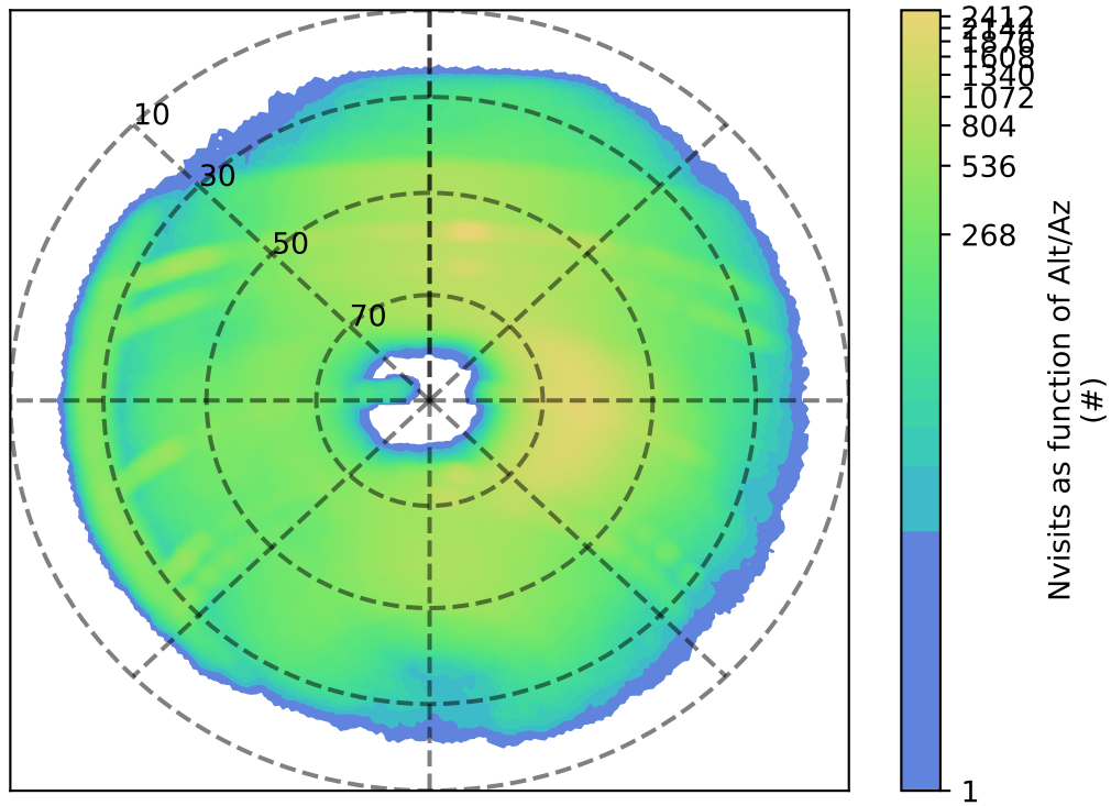
too_combined_s0.0_v3.4_10yrs r: Nvisits as function of Alt/Az
