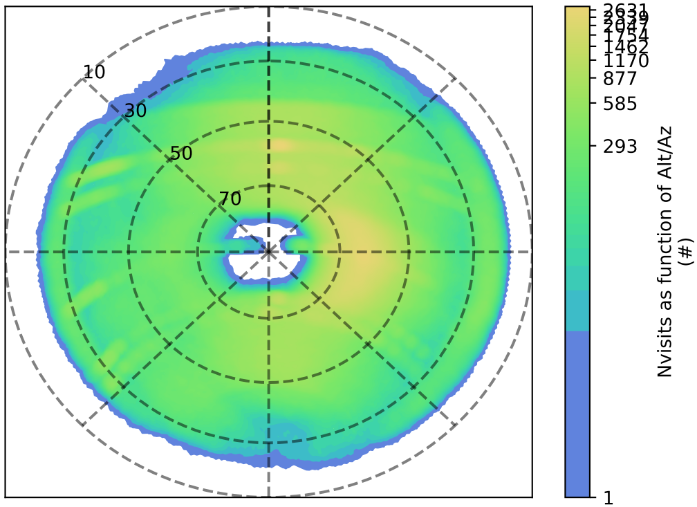
too_combined_s0.0_v3.4_10yrs i: Nvisits as function of Alt/Az
