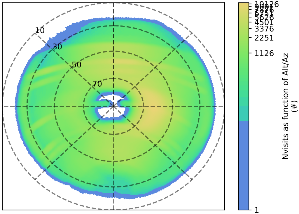
too_combined_s0.0_v3.4_10yrs : Nvisits as function of Alt/Az
