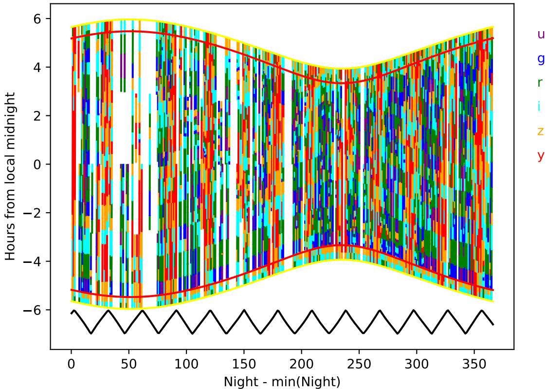
too_combined_s0.0_v3.4_10yrs year 9-10: Hourglass
