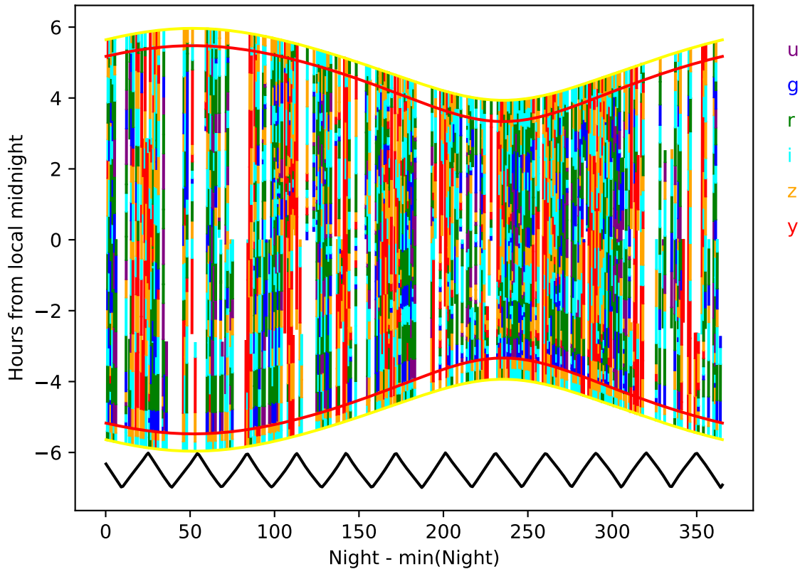
too_combined_s0.0_v3.4_10yrs year 7-8: Hourglass
